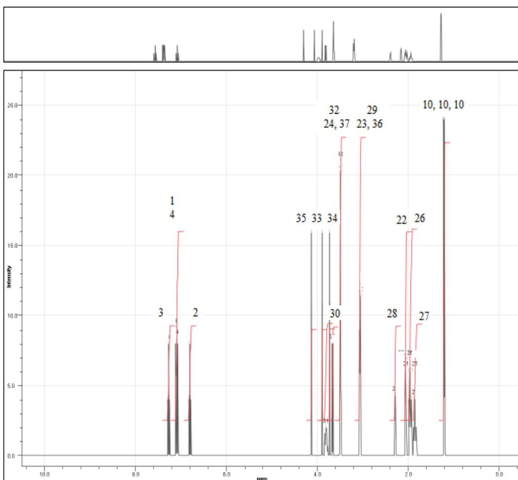
Figure 53: Better resolution of ^1\text{H} -NMR spectrum of (AZ-5) by Marvin Sketch.
